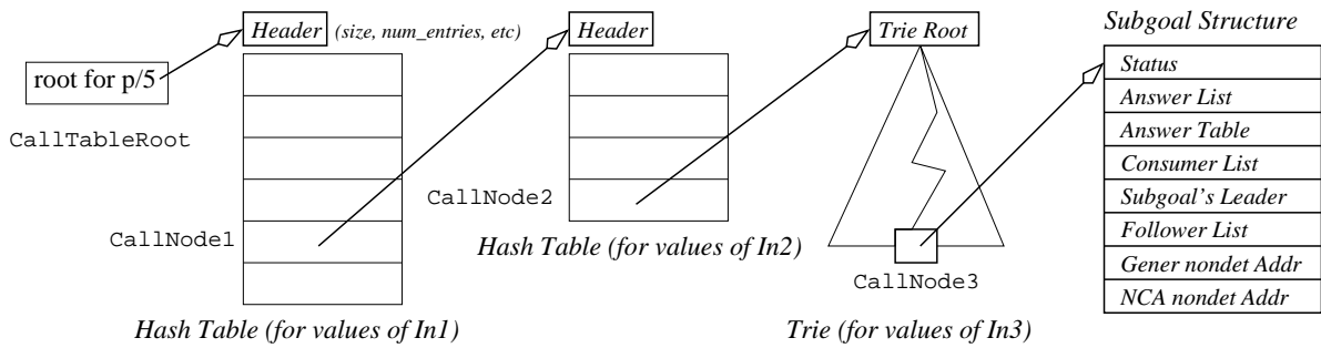
Figure 1: Data structures created for the calls of predicate p/5
